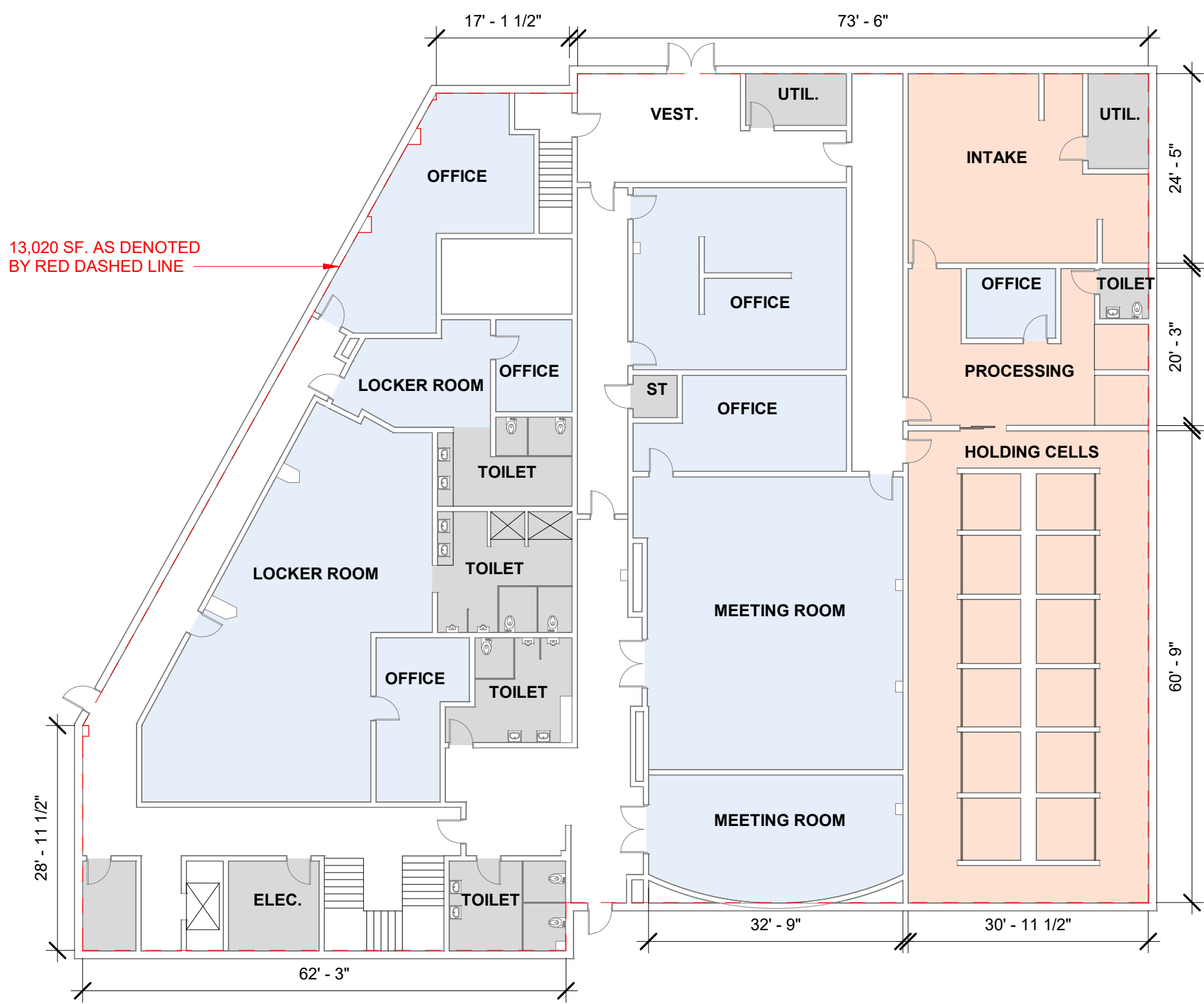
9TH DISTRICT POLICE STATION - FLOOR PLAN A 1/16" = 1'-0" 1
