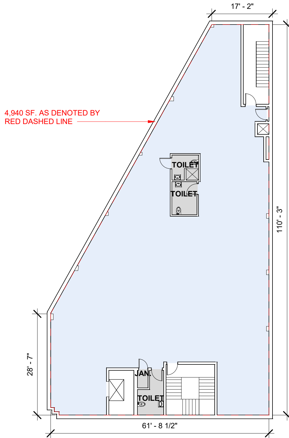
9TH DISTRICT POLICE STATION - FLOOR PLAN B2 1/16" = 1'-0"
