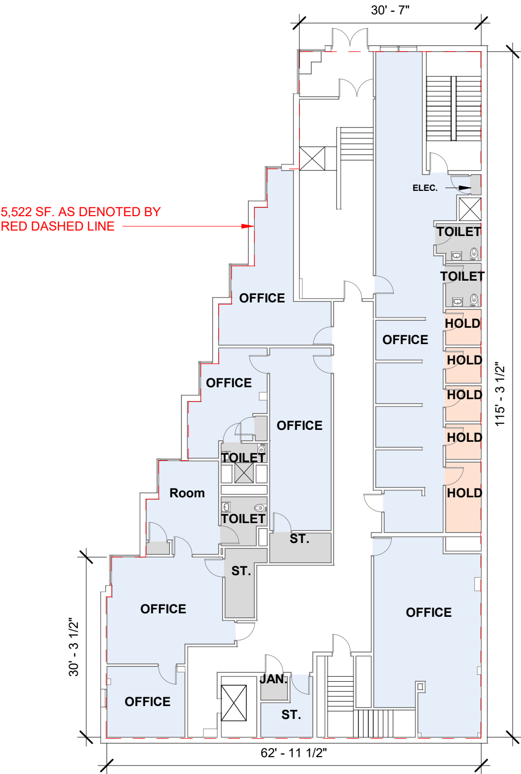
9TH DISTRICT POLICE STATION - FLOOR PLAN C 1/16" = 1'-0" 1
