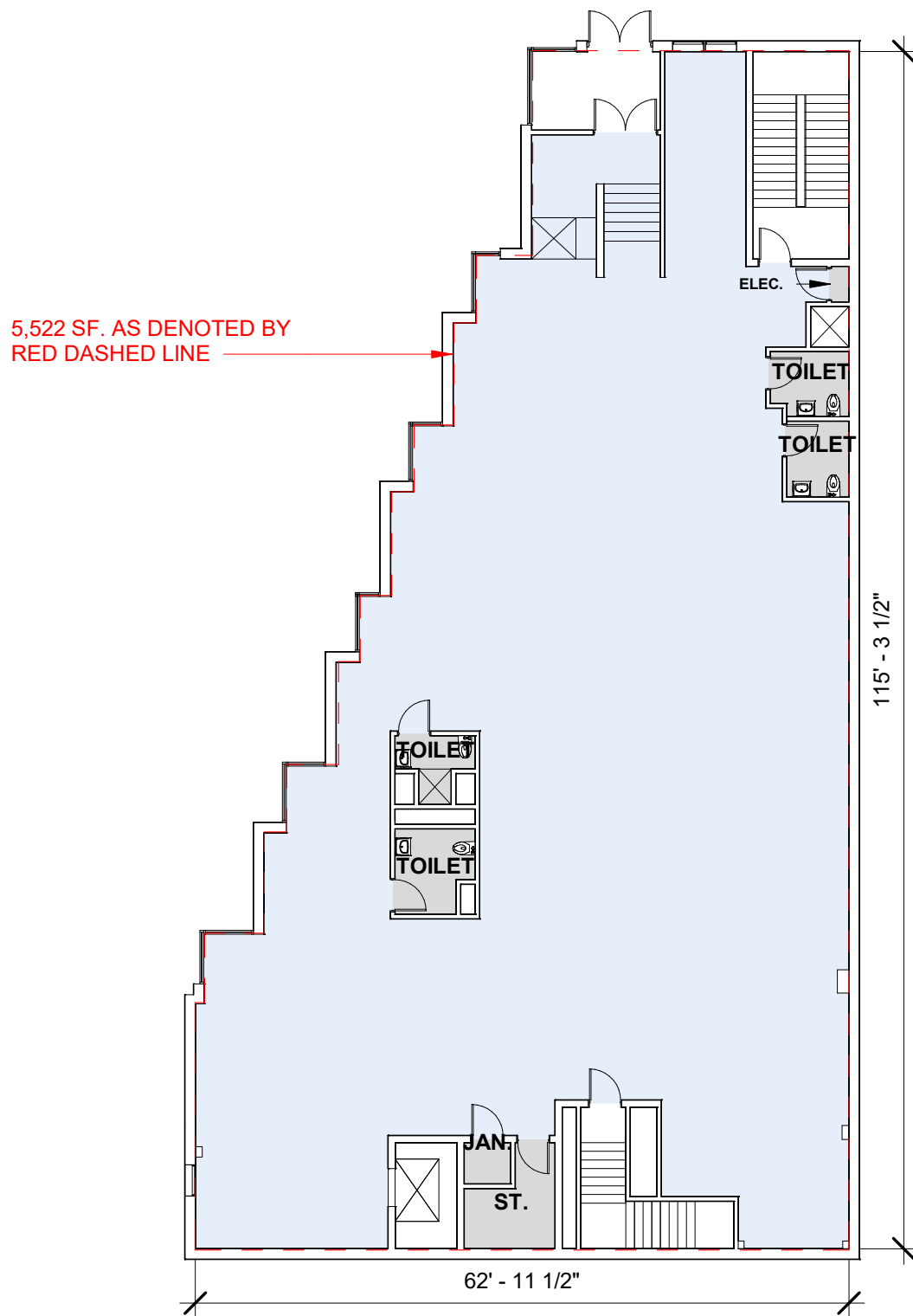
9TH DISTRICT POLICE STATION - FLOOR PLAN C2 1/16" = 1'-0"
