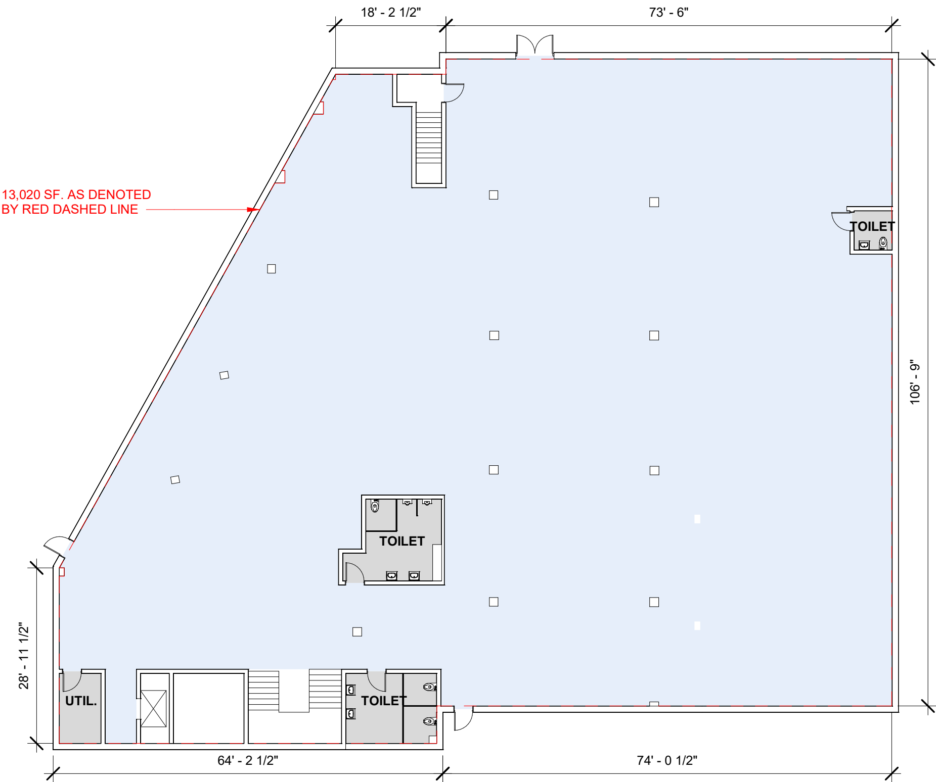
9TH DISTRICT POLICE STATION - FLOOR PLAN A2 1/16" = 1'-0"
